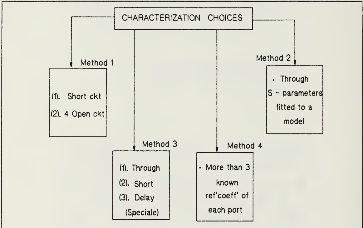
Figure 2. The Four Main Choices of N.A.-Fixturing Characterization.
