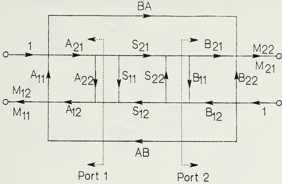
Figure 11. Signal Flow Graph for Measurements on a Two - Port Network
