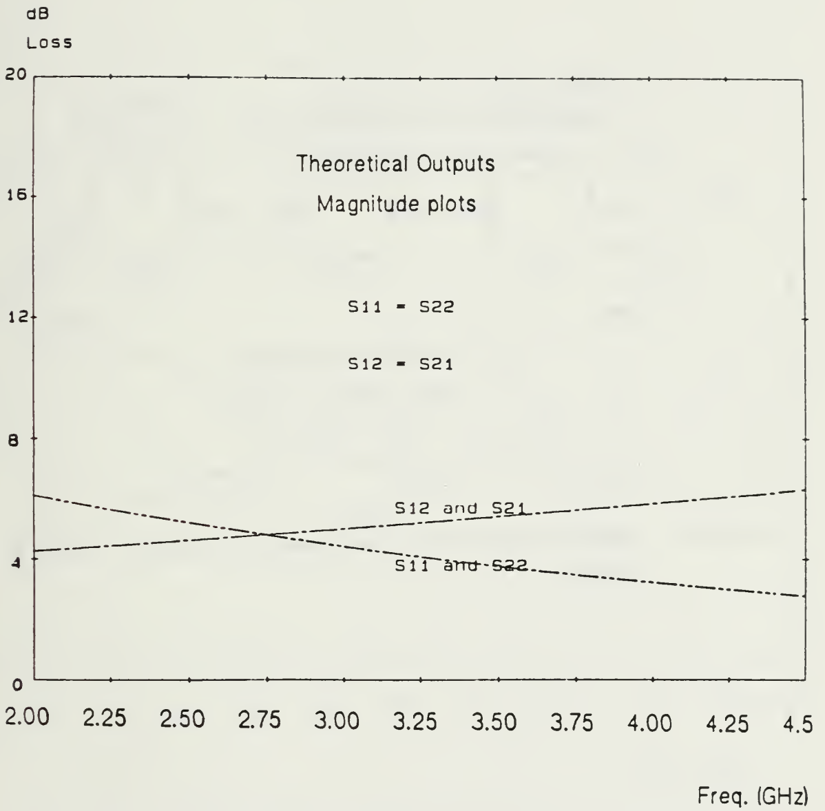
Figure 15. Theoretical Scattering Parameters of 51 Ohm Resistor
